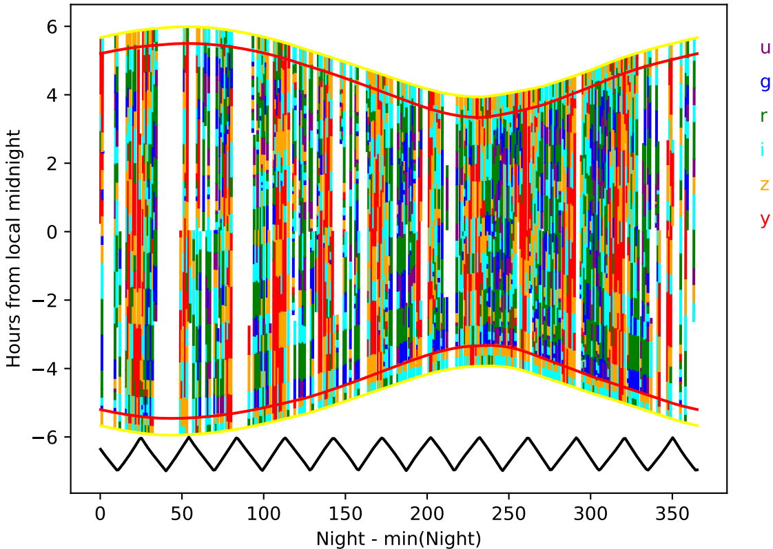
internal_u_expt27_nscale1.1v3.4_10yrs year 4-5: Hourglass
