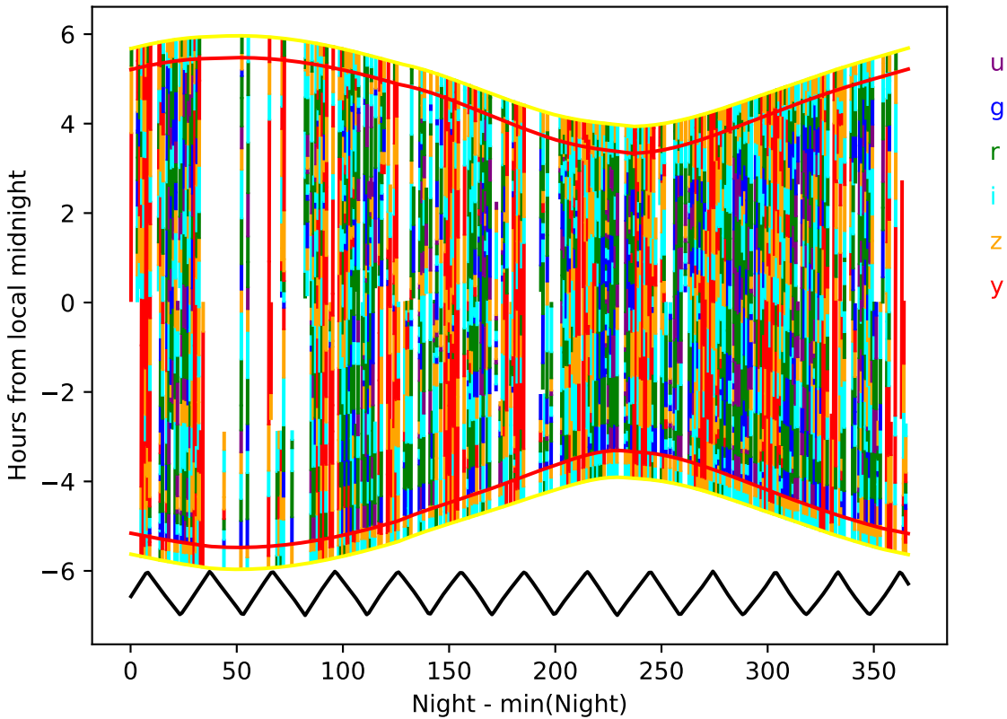
internal_u_expt27_nscale1.1v3.4_10yrs year 3-4: Hourglass
