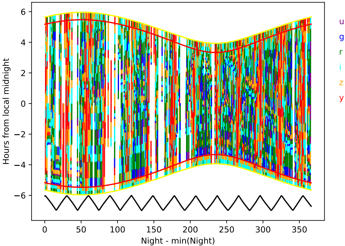
internal_u_expt27_nscale1.1v3.4_10yrs year 1-2: Hourglass
