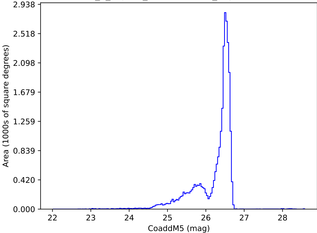
internal_u_expt27_nscale1.1v3.4_10yrs i: CoaddM5
