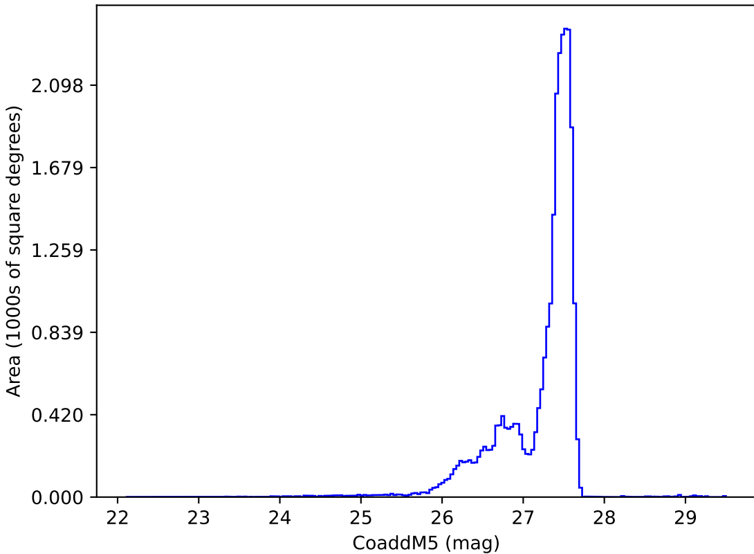
internal_u_expt27_nscale1.1v3.4_10yrs : CoaddM5
