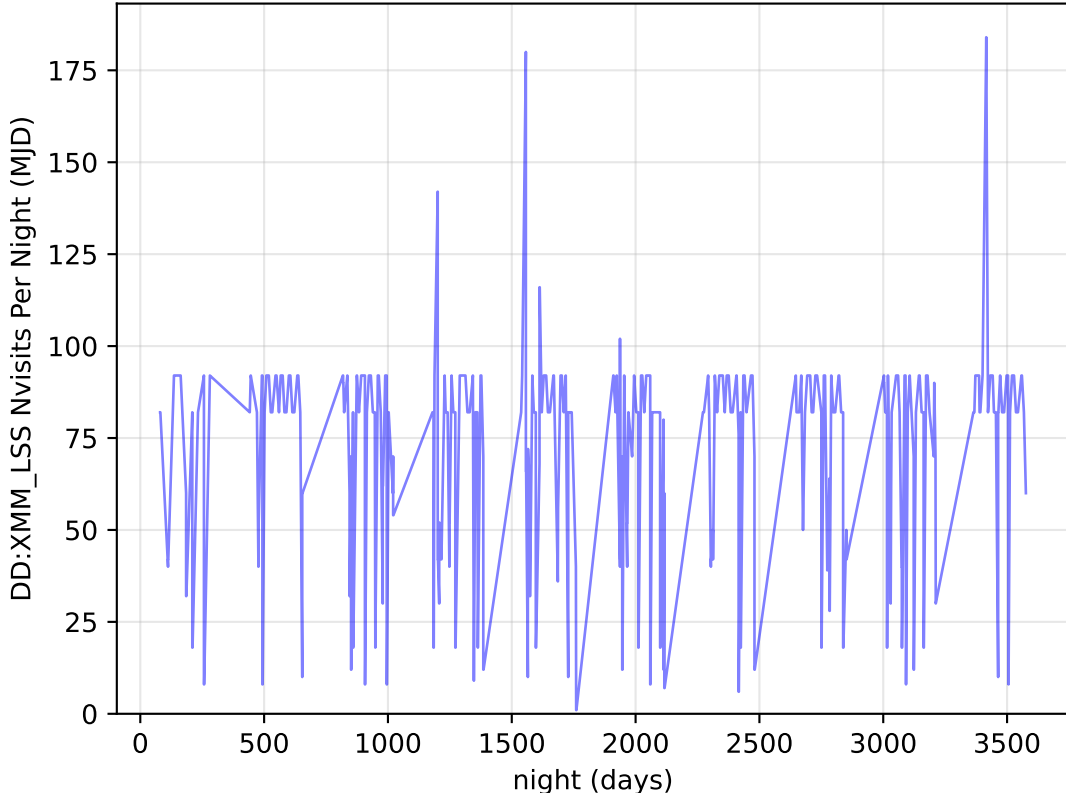
internal_u_expt27_nscale1.1v3.4_10yrs all bands: DD:XMM_LSS Nvisits Per Night
