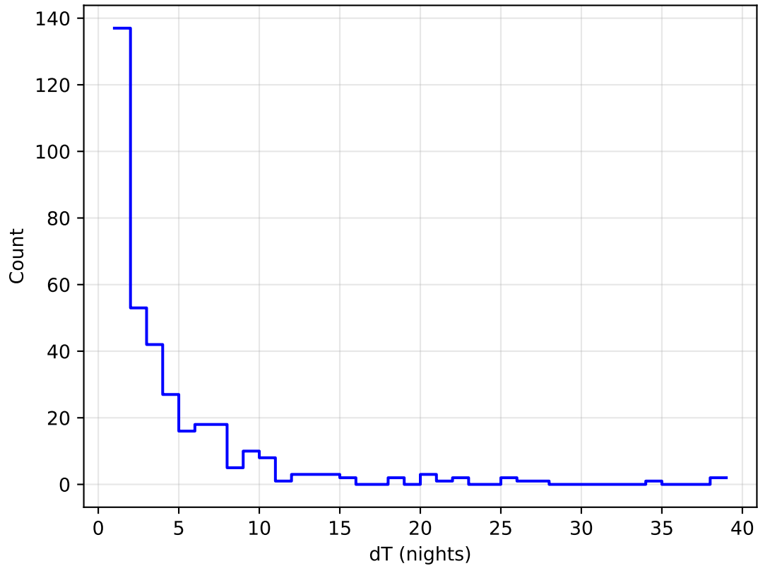
internal_u_expt27_nscale1.1v3.4_10yrs all bands: DD:WFD Delta Nights Histogram
