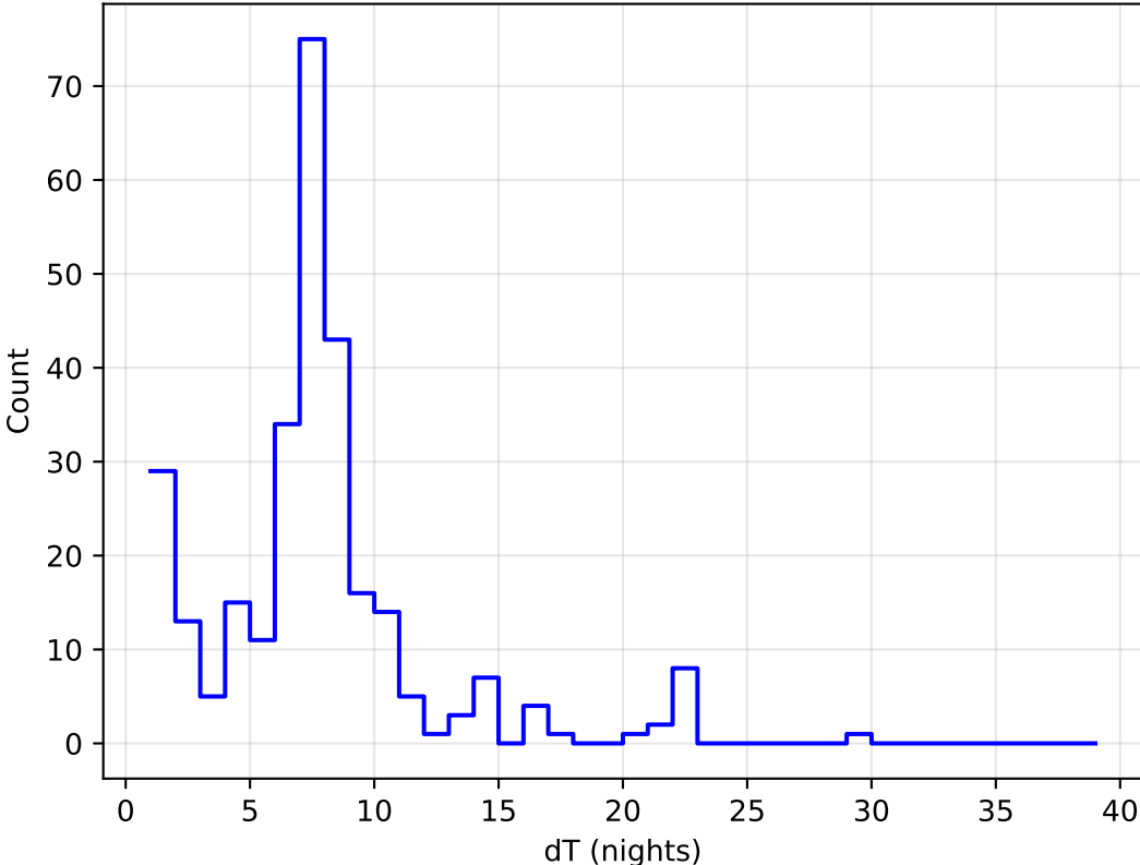
internal_u_expt27_nscale1.1v3.4_10yrs all bands: DD:EDFS Delta Nights Histogram
