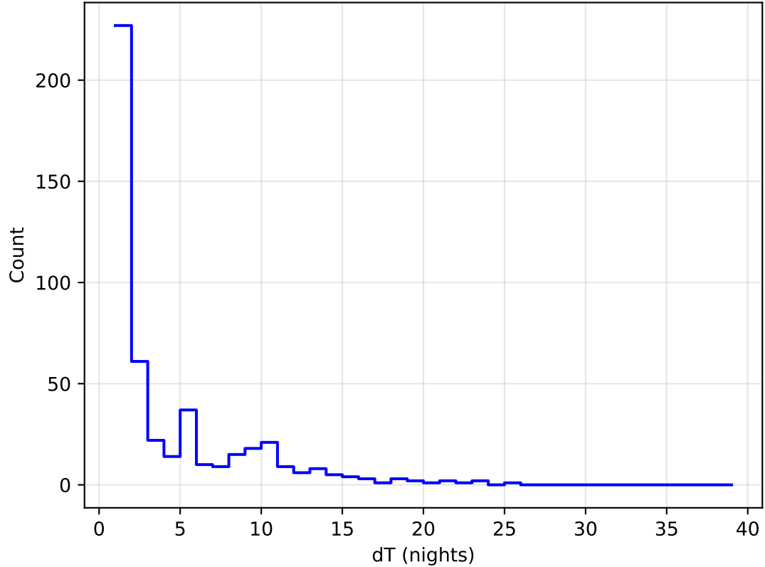
internal_u_expt27_nscale1.1v3.4_10yrs all bands: DD:COSMOS Delta Nights Histogram
