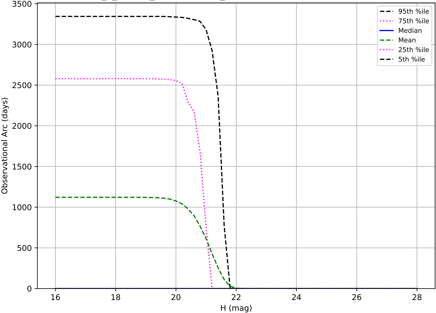
internal_u_expt27_nscale1.0v3.4_10yrs: Observational Arc Length Vatra
