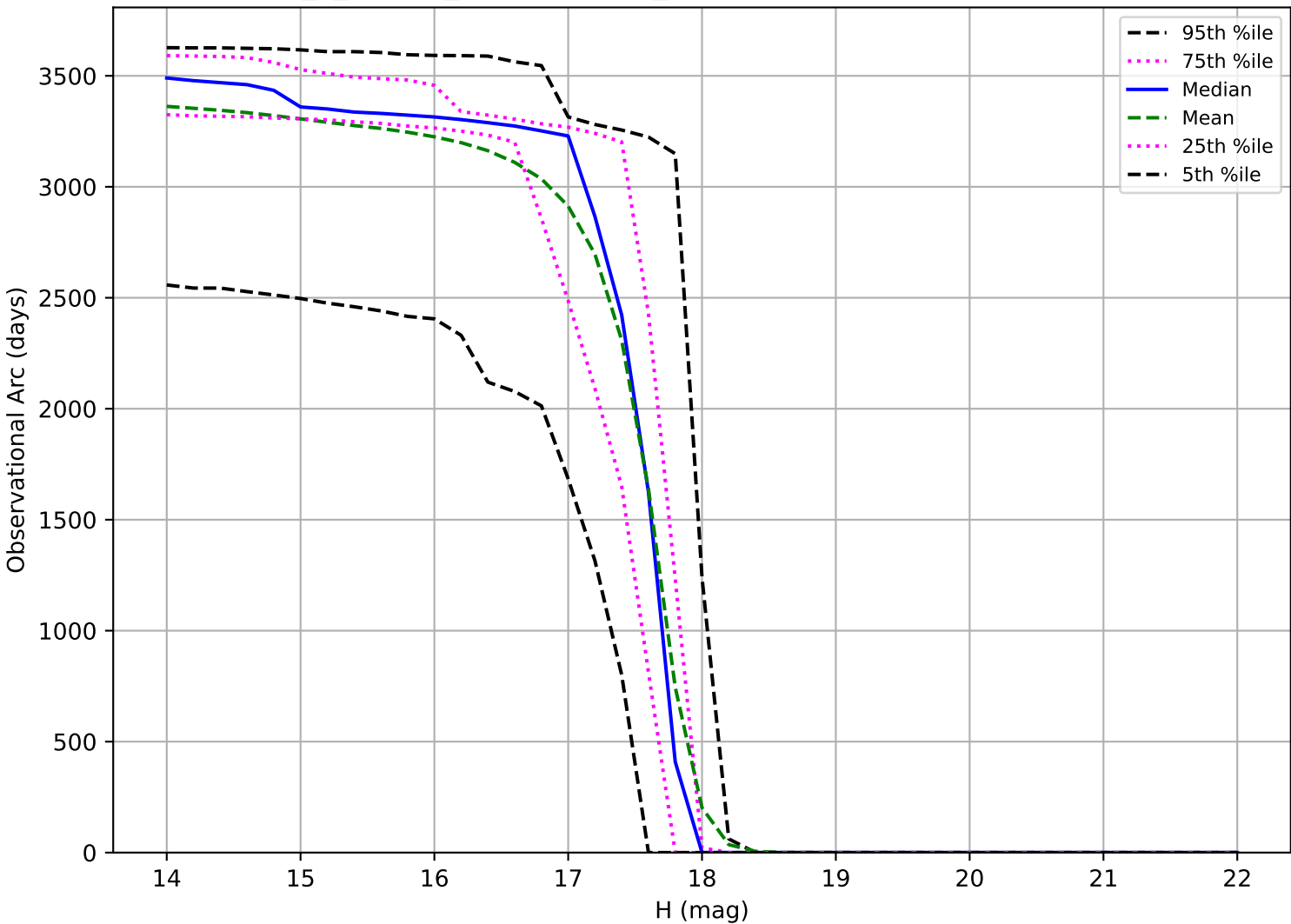
internal_u_expt27_nscale1.0v3.4_10yrs: Observational Arc Length Trojan
