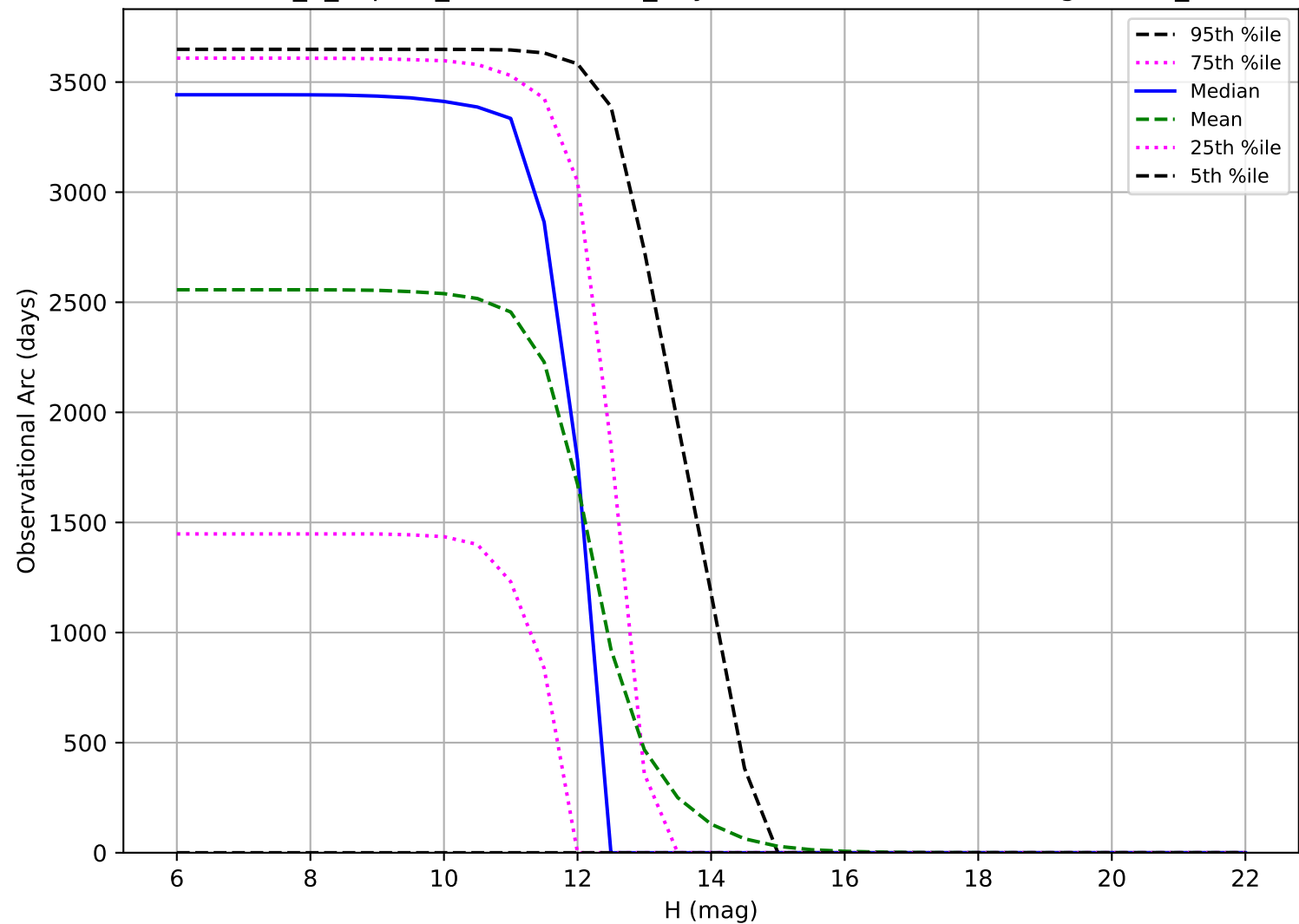
internal_u_expt27_nscale1.0v3.4_10yrs: Observational Arc Length OCC_r20
