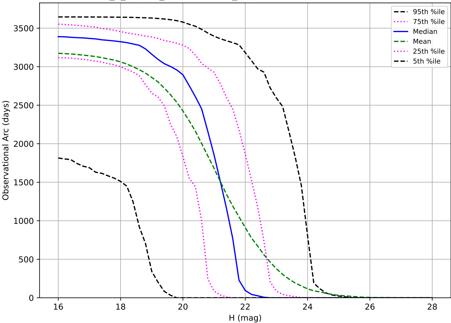
internal_u_expt27_nscale1.0v3.4_10yrs: Observational Arc Length NEO
