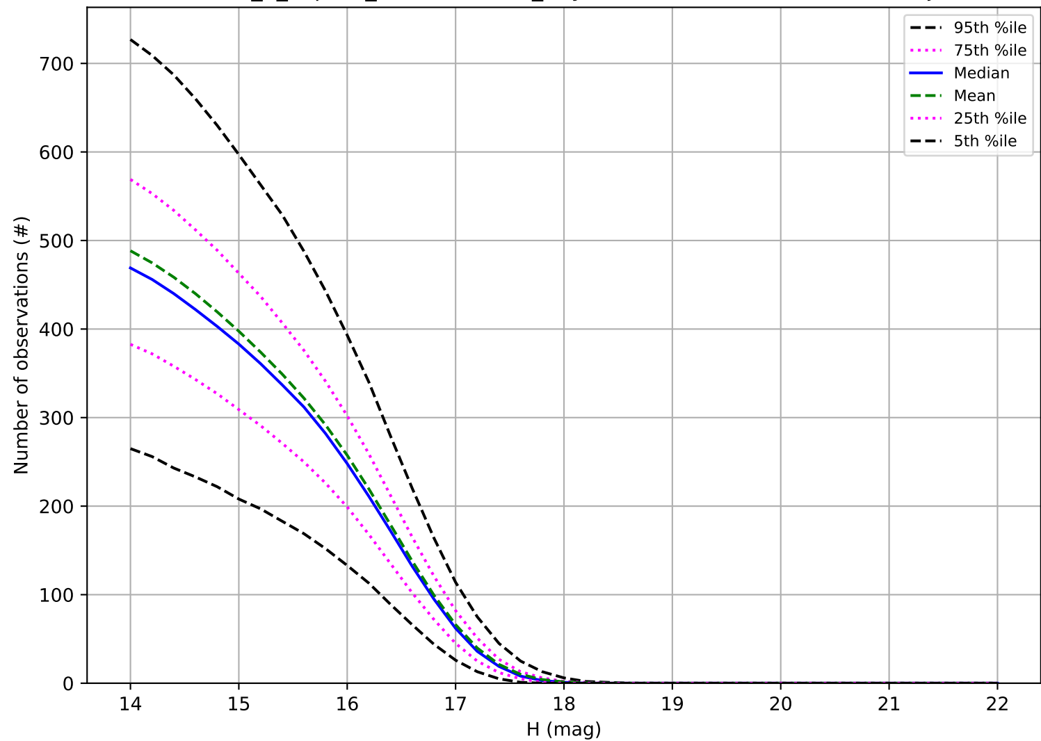
internal_u_expt27_nscale1.0v3.4_10yrs: Number of observations Trojan
