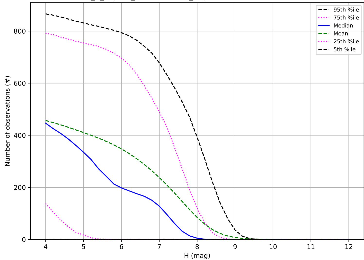
internal_u_expt27_nscale1.0v3.4_10yrs: Number of observations TNO
