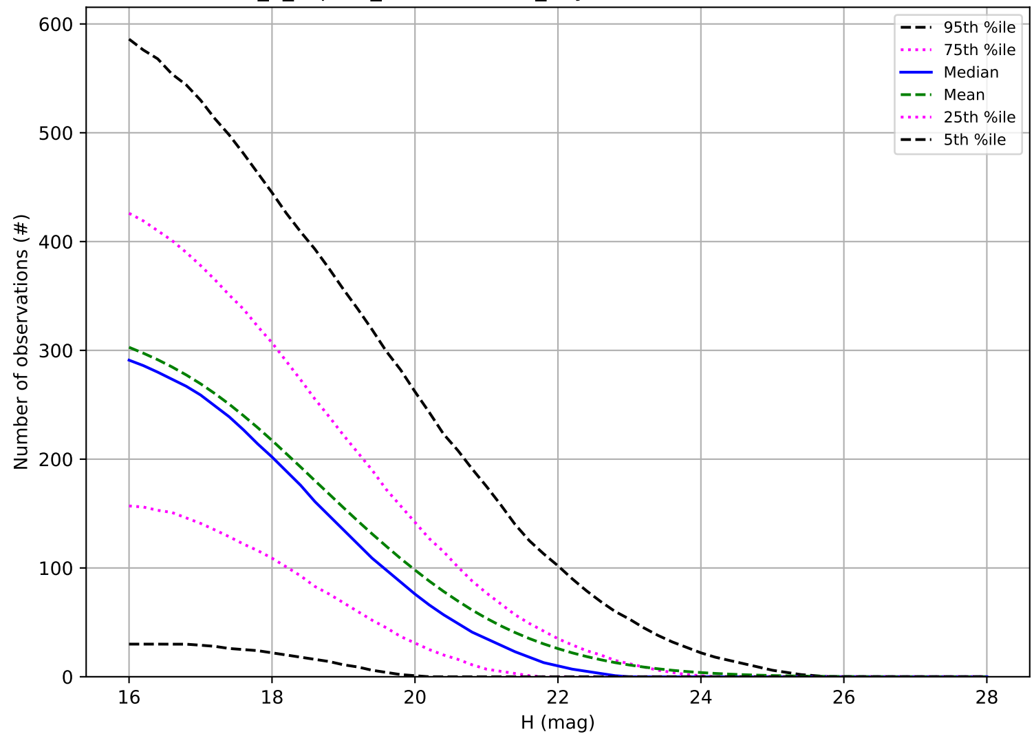
internal_u_expt27_nscale1.0v3.4_10yrs: Number of observations NEO
