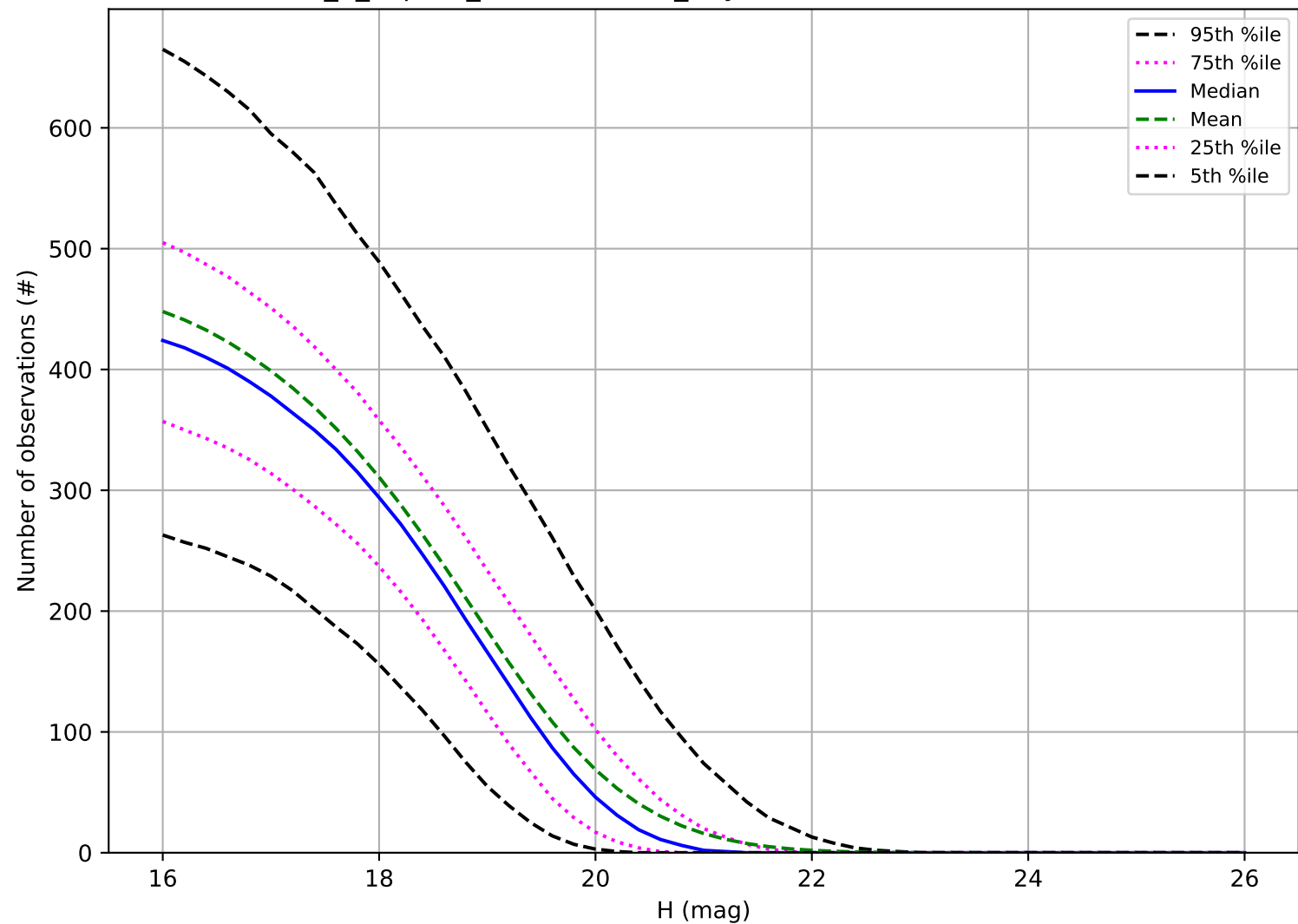
internal_u_expt27_nscale1.0v3.4_10yrs: Number of observations MBA
