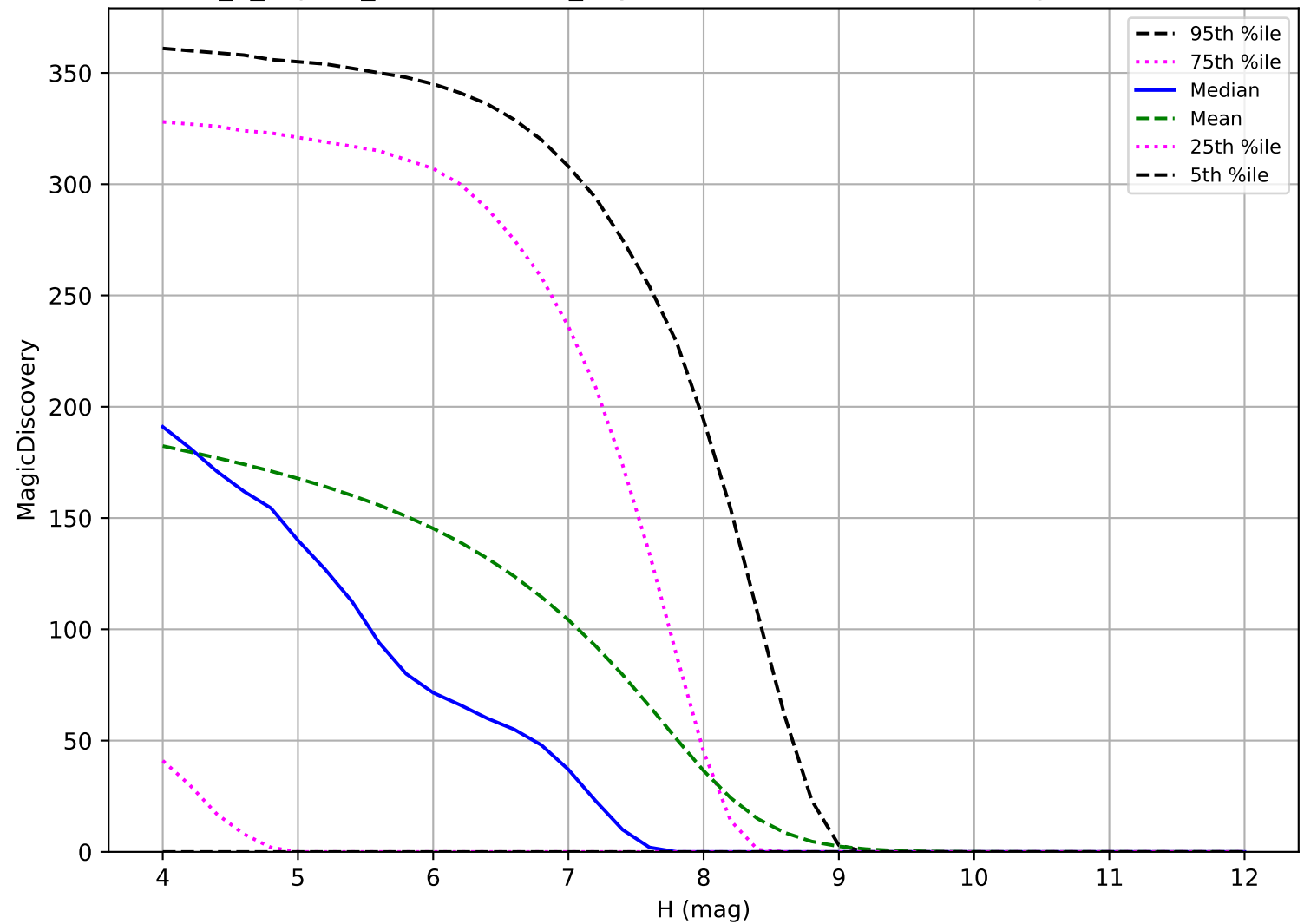
internal_u_expt27_nscale1.0v3.4_10yrs: TNO 6 detections in 60 nights detection loss
