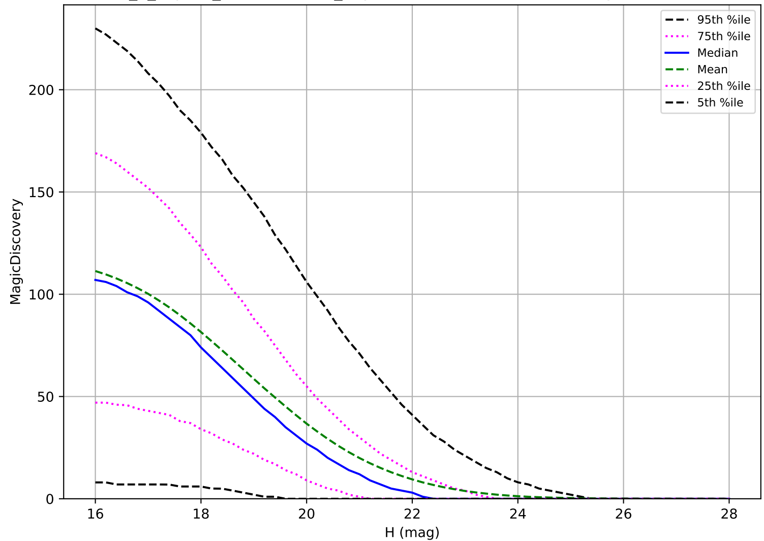
internal_u_expt27_nscale1.0v3.4_10yrs: PHA 6 detections in 60 nights detection loss
