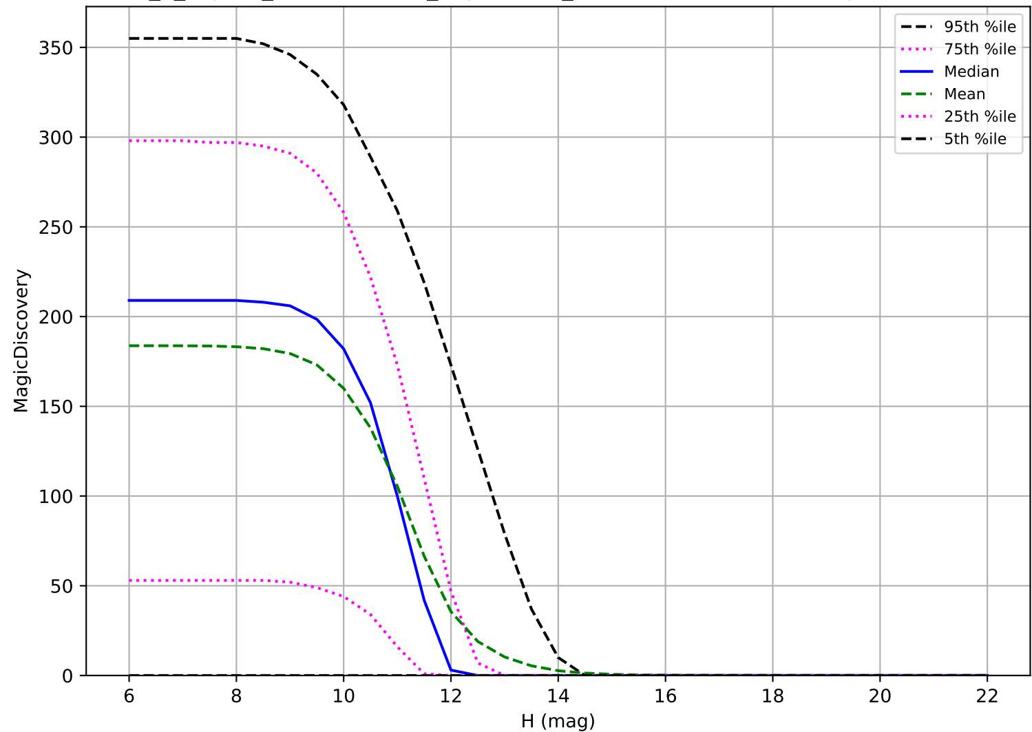
internal_u_expt27_nscale1.0v3.4_10yrs: OCC_r20 6 detections in 60 nights detection loss
