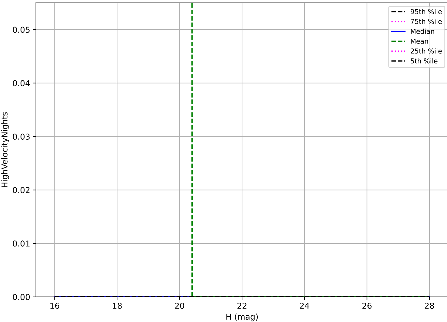
internal_u_expt27_nscale1.0v3.4_10yrs: Vatira High velocity pair detection loss
