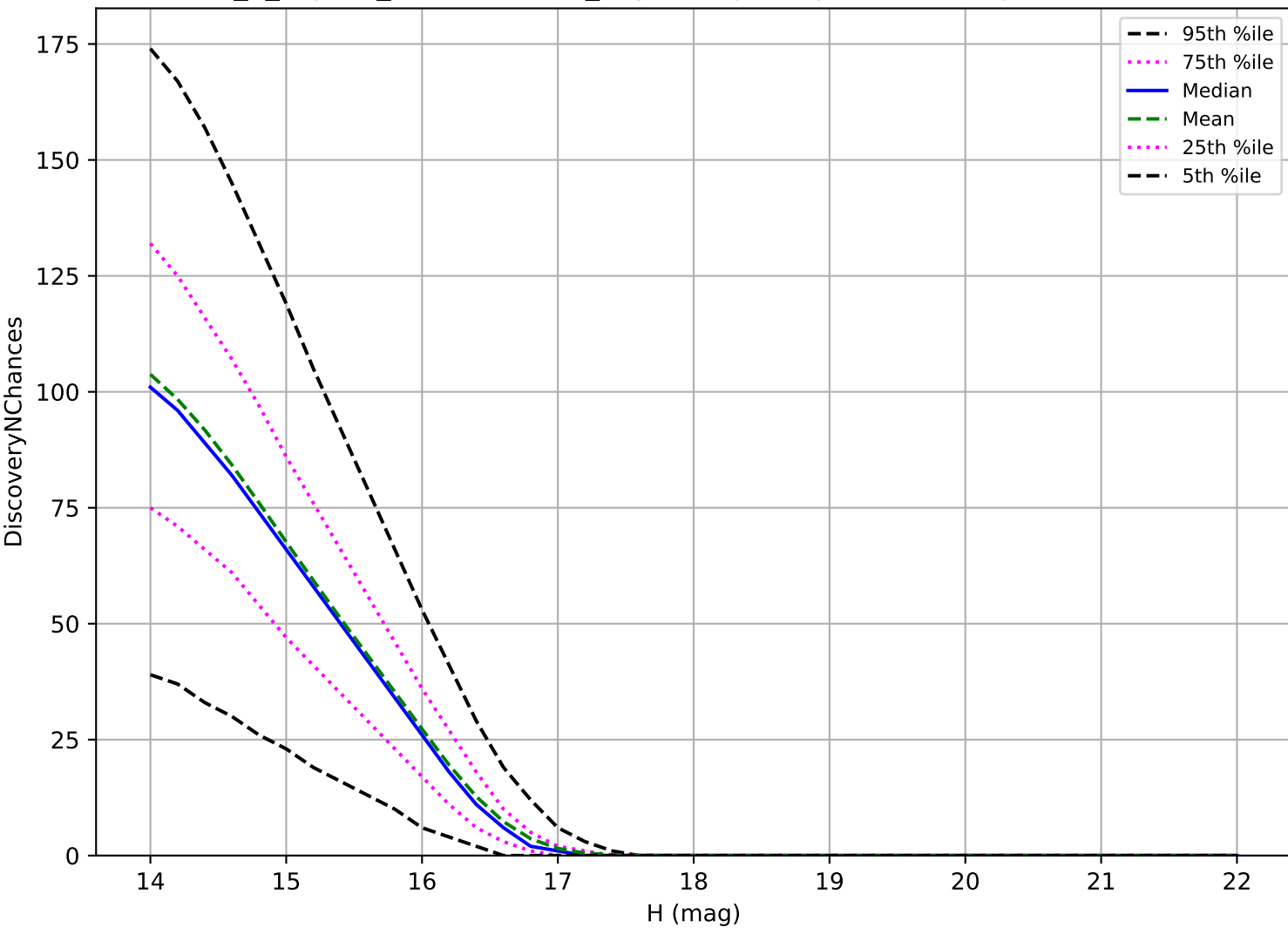
internal_u_expt27_nscale1.0v3.4_10yrs: Trojan 3 pairs in 15 nights detection loss
