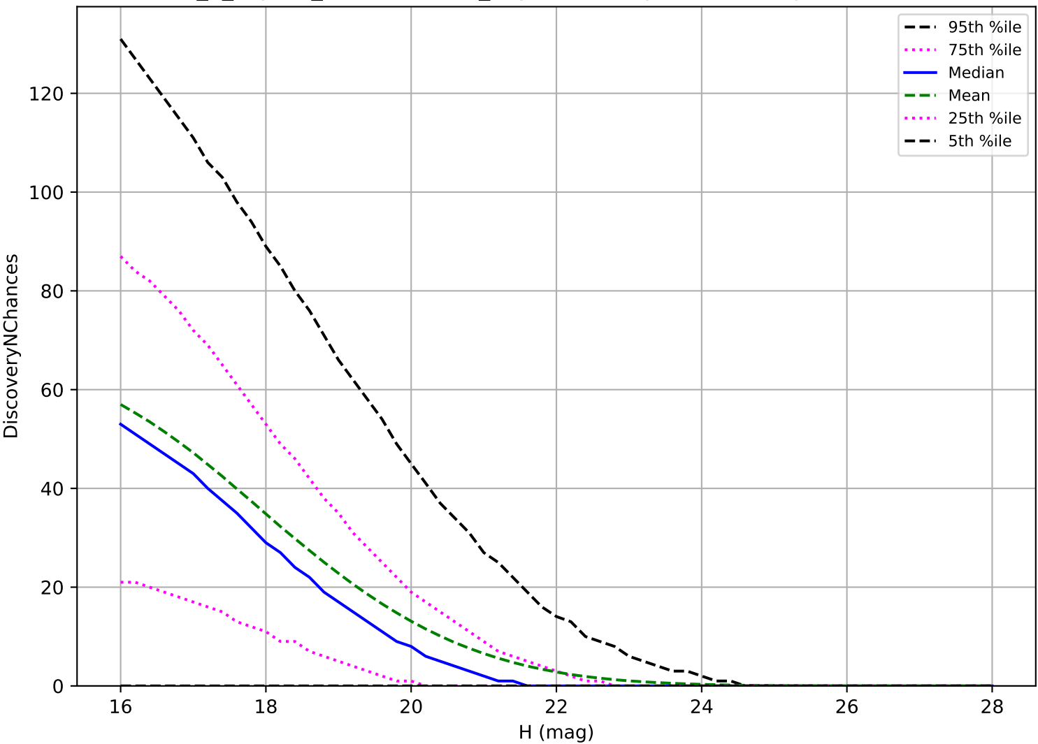
internal_u_expt27_nscale1.0v3.4_10yrs: NEO 3 pairs in 15 nights detection loss
