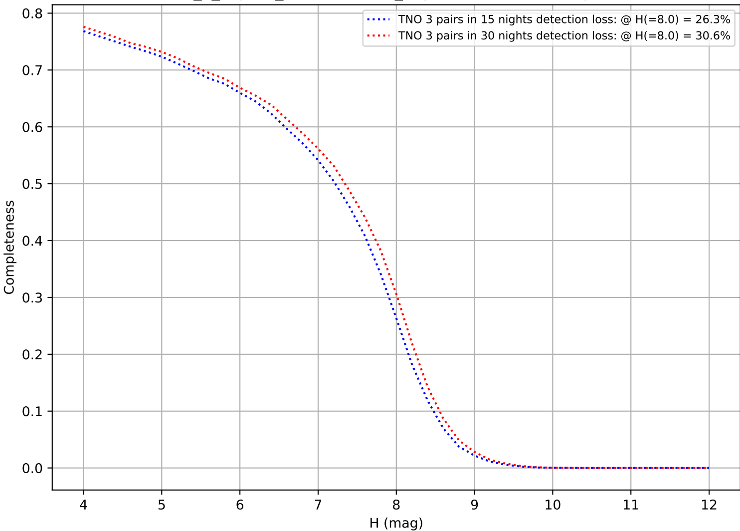
internal_u_expt27_nscale1.0v3.4_10yrs: DifferentialCompleteness
