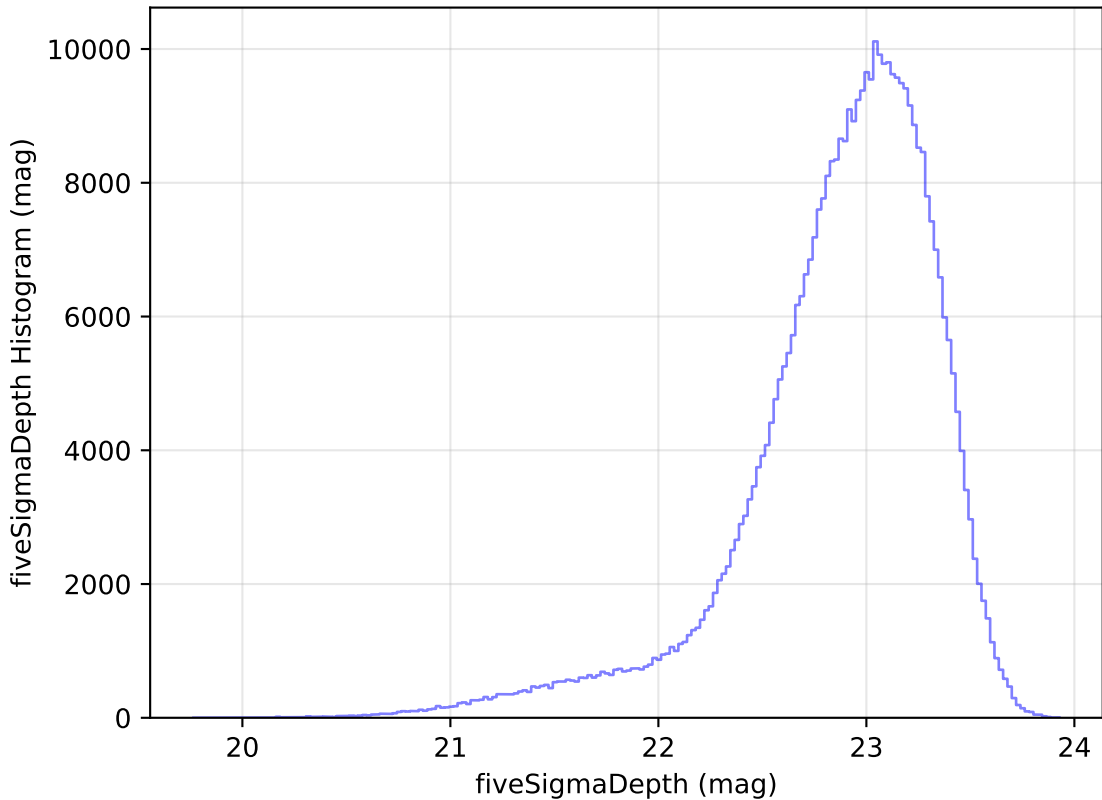
internal_u_expt27_nscale1.0v3.4_10yrs z: fiveSigmaDepth Histogram
