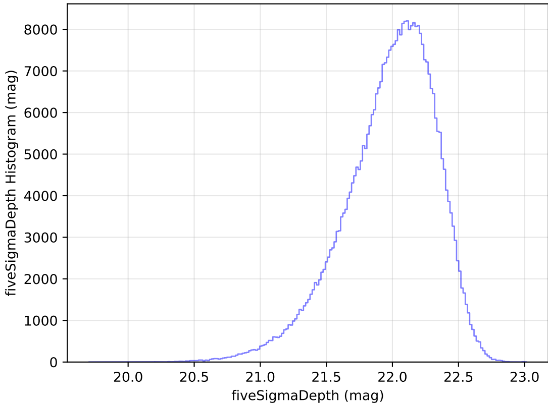
internal_u_expt27_nscale1.0v3.4_10yrs y: fiveSigmaDepth Histogram
