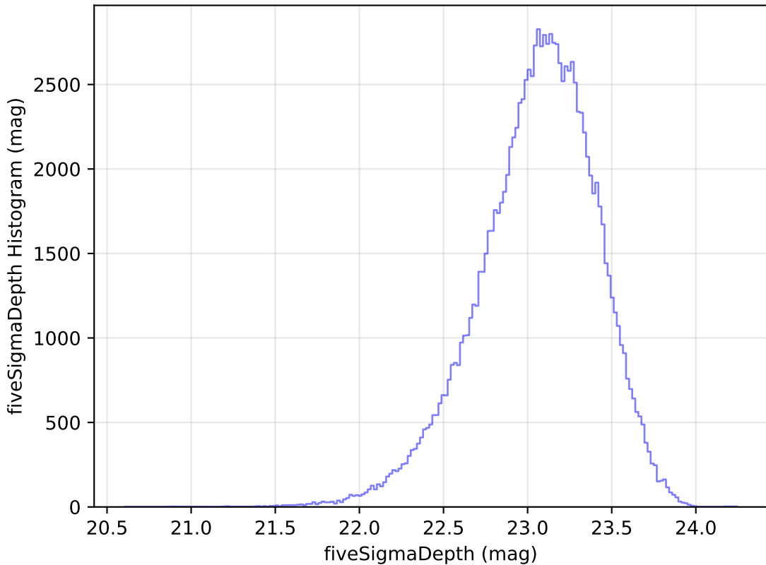
internal_u_expt27_nscale1.0v3.4_10yrs u: fiveSigmaDepth Histogram
