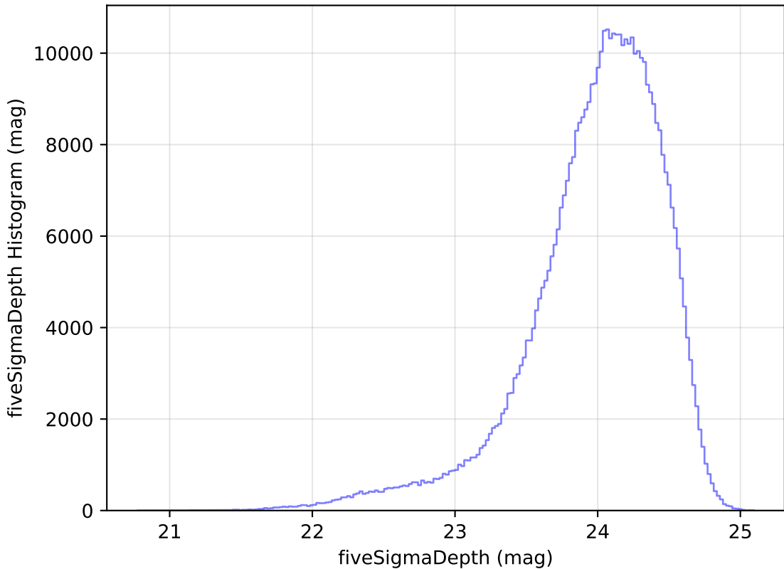
internal_u_expt27_nscale1.0v3.4_10yrs r: fiveSigmaDepth Histogram
