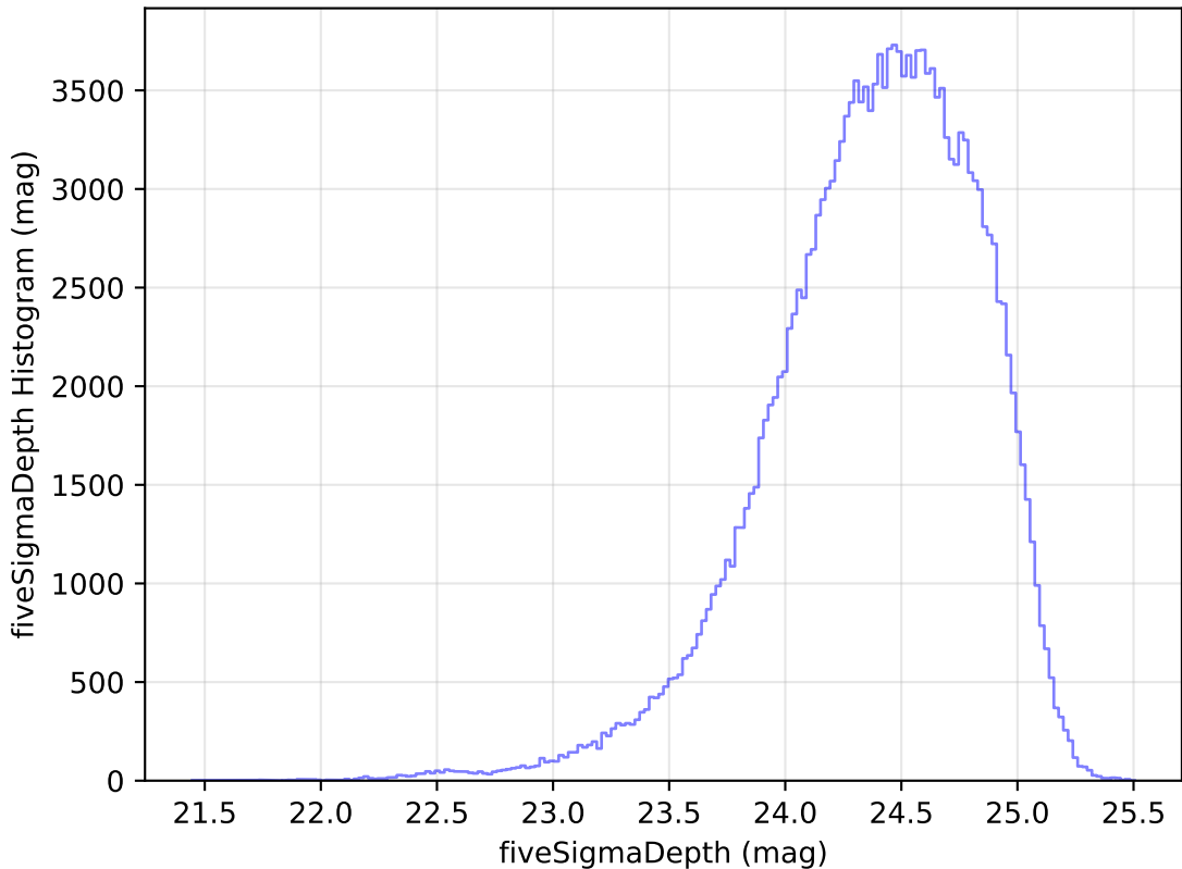
internal_u_expt27_nscale1.0v3.4_10yrs g: fiveSigmaDepth Histogram
