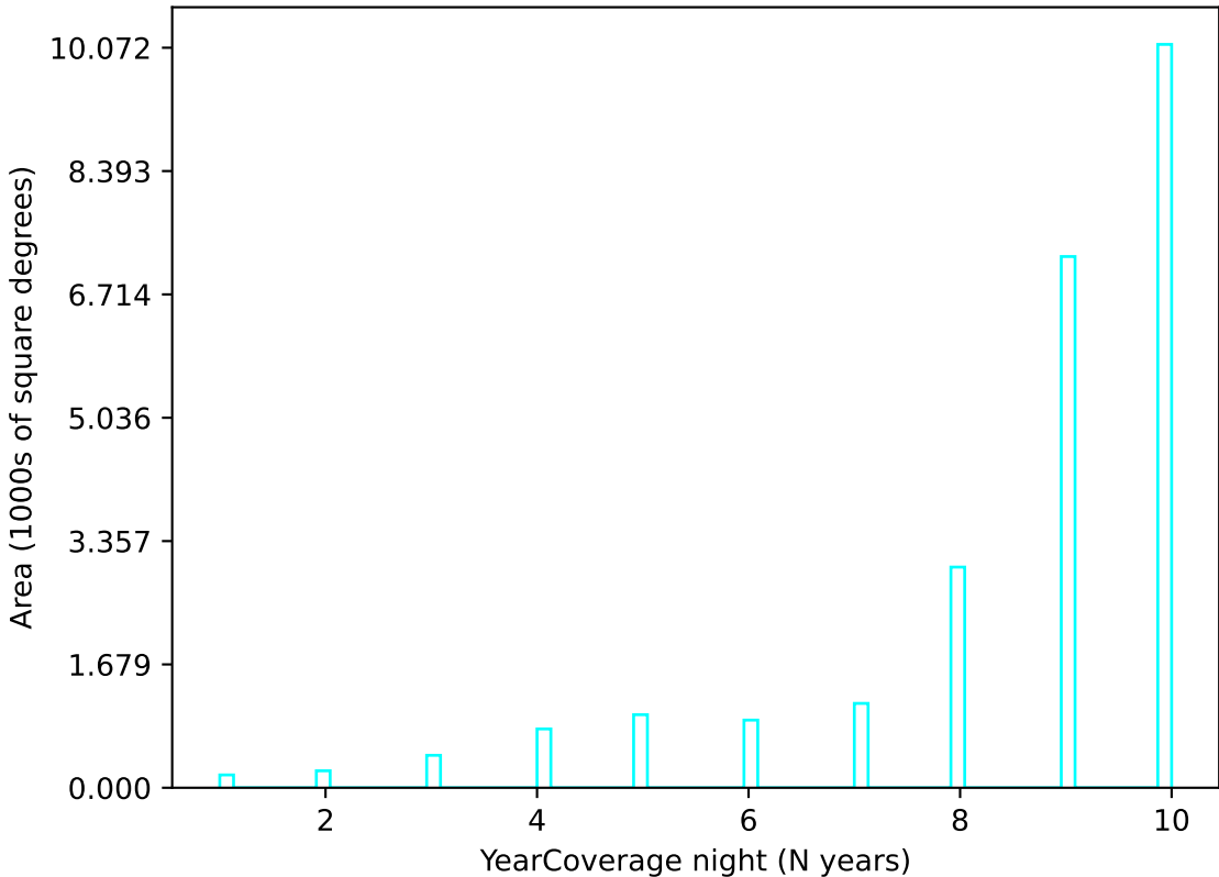
internal_u_expt27_nscale1.0v3.4_10yrs u band: YearCoverage night
