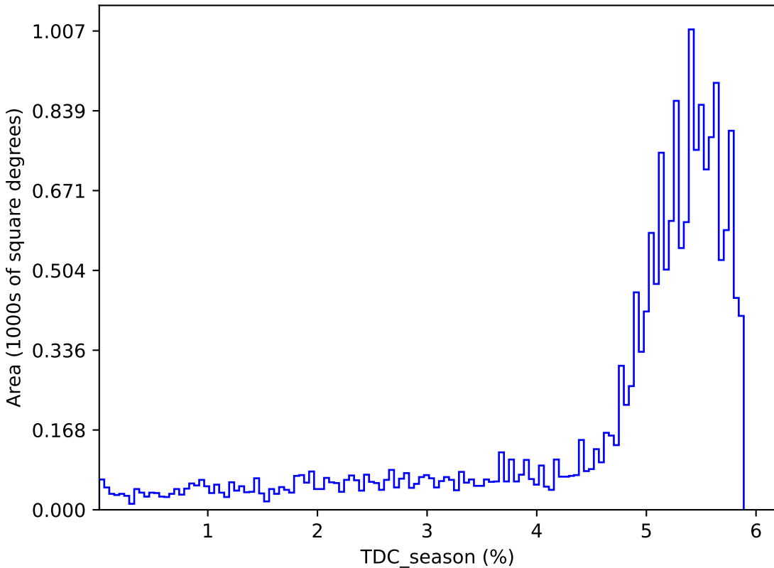
internal_u_expt27_nscale1.0v3.4_10yrs : TDC_season
