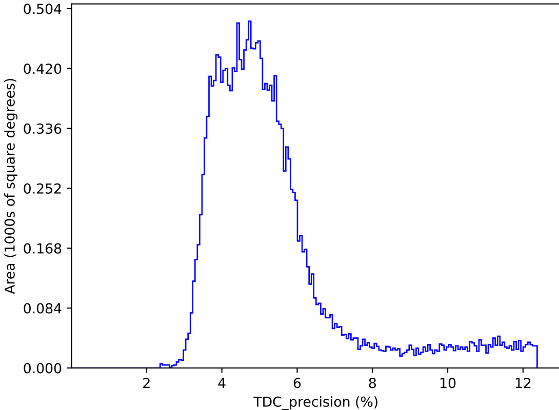
internal_u_expt27_nscale1.0v3.4_10yrs : TDC_precision
