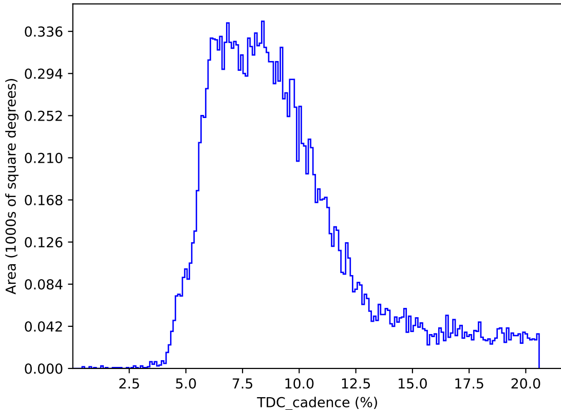
internal_u_expt27_nscale1.0v3.4_10yrs : TDC_cadence
