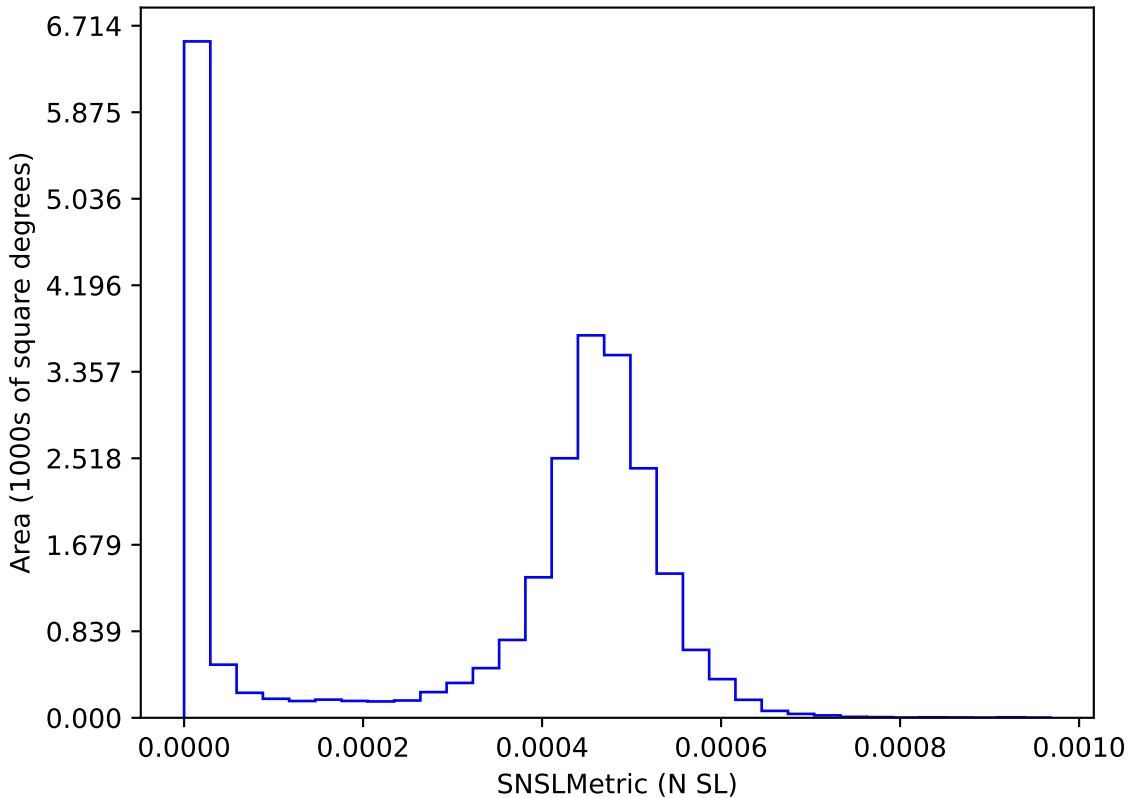
internal_u_expt27_nscale1.0v3.4_10yrs : SNSLMetric
