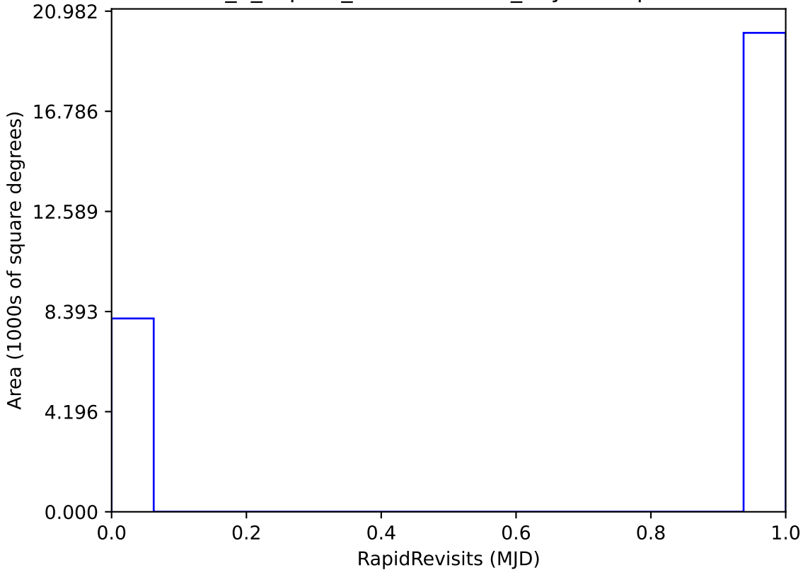
internal_u_expt27_nscale1.0v3.4_10yrs : RapidRevisits
