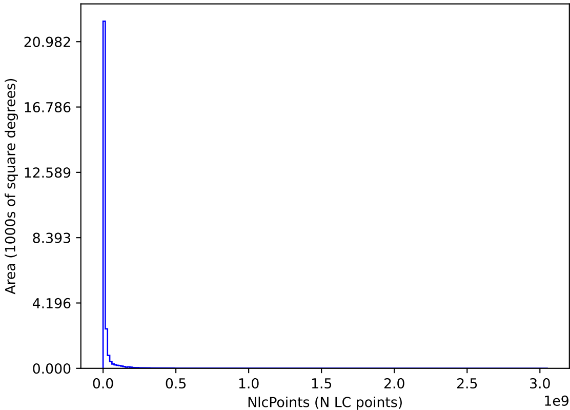
internal_u_expt27_nscale1.0v3.4_10yrs : NlcPoints
