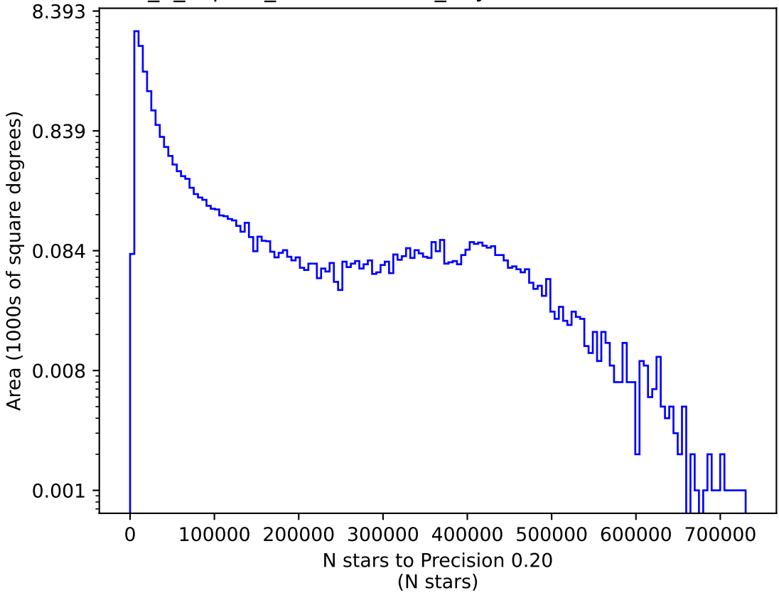
internal_u_expt27_nscale1.0v3.4_10yrs i: N stars to Precision 0.20
