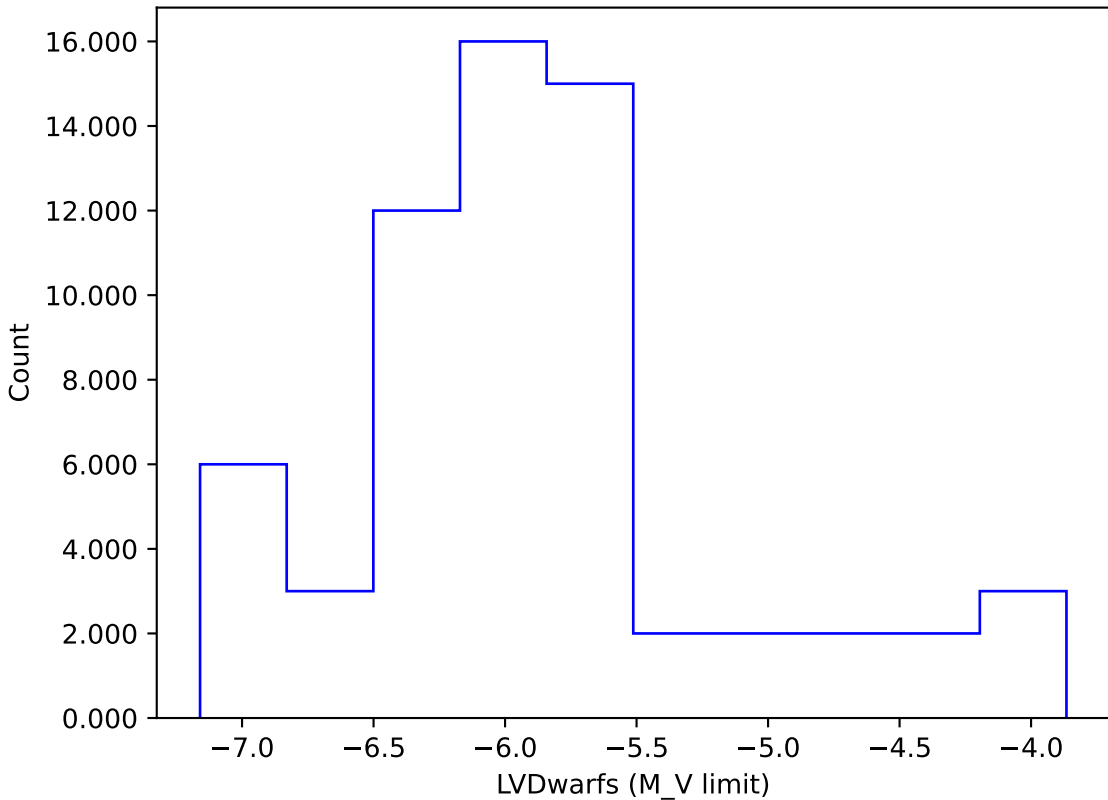
internal_u_expt27_nscale1.0v3.4_10yrs gi: LVDwarfs
