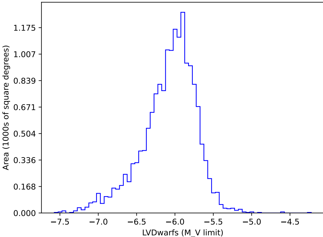
internal_u_expt27_nscale1.0v3.4_10yrs gi: LVDwarfs
