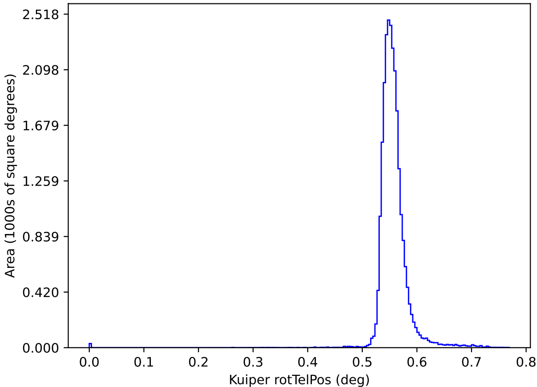
internal_u_expt27_nscale1.0v3.4_10yrs y: Kuiper rotTelPos
