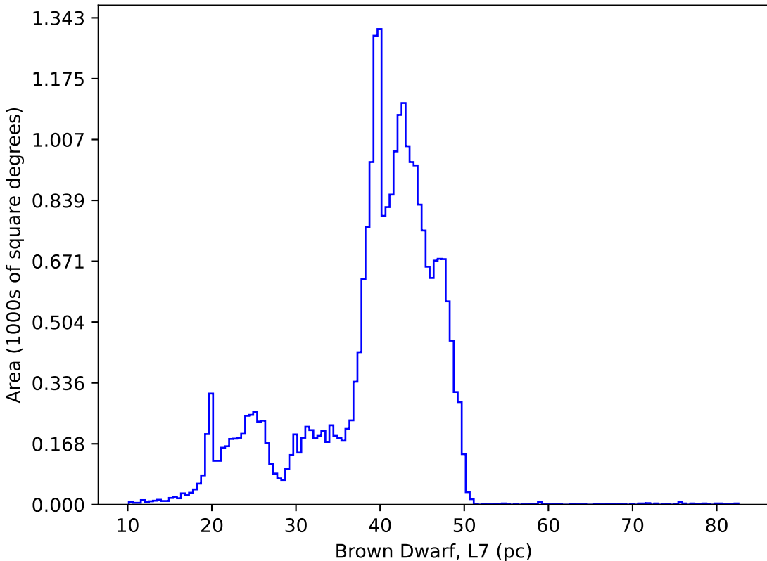
internal_u_expt27_nscale1.0v3.4_10yrs : Brown Dwarf, L7
