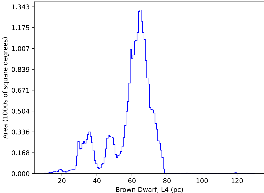
internal_u_expt27_nscale1.0v3.4_10yrs : Brown Dwarf, L4
