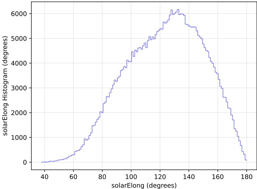
internal_u_expt27_nscale1.0v3.4_10yrs WFD y band: solarElong Histogram
