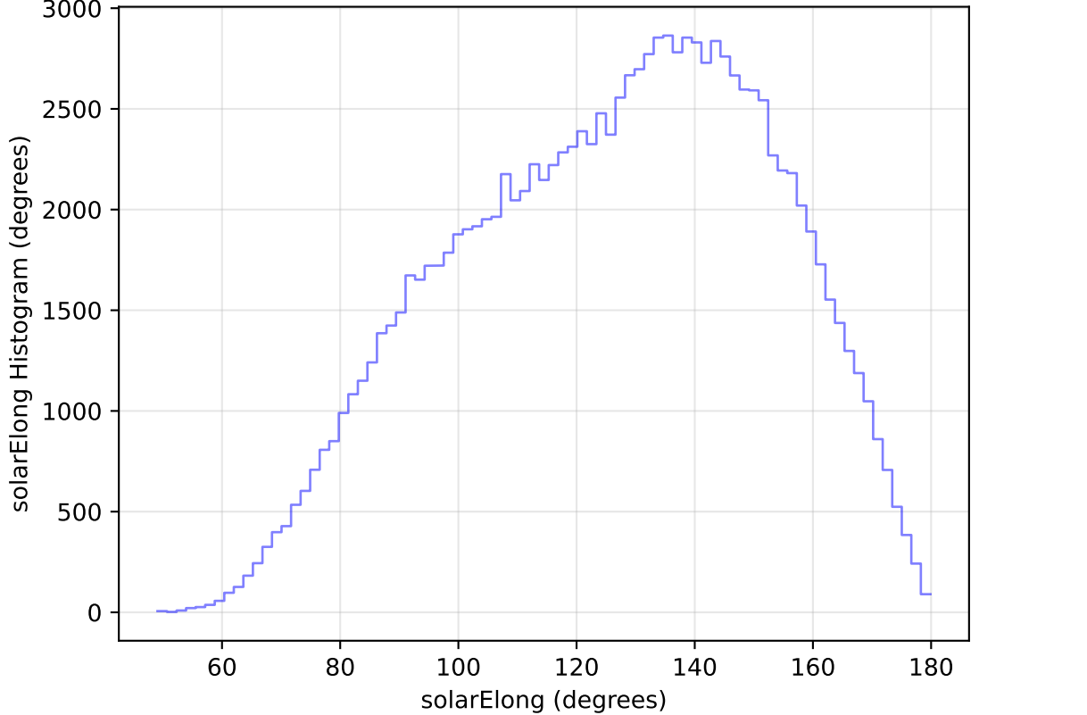
internal_u_expt27_nscale1.0v3.4_10yrs WFD u band: solarElong Histogram
