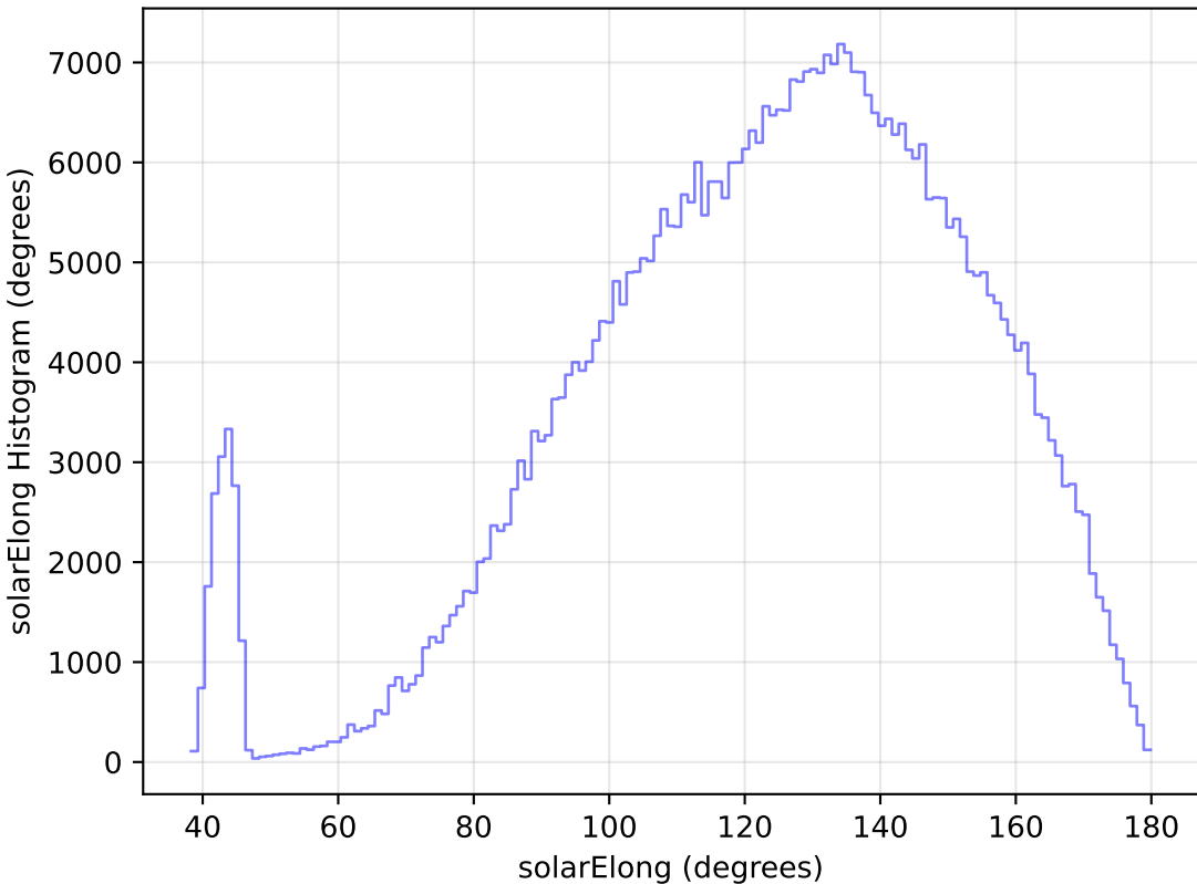
internal_u_expt27_nscale1.0v3.4_10yrs WFD r band: solarElong Histogram
