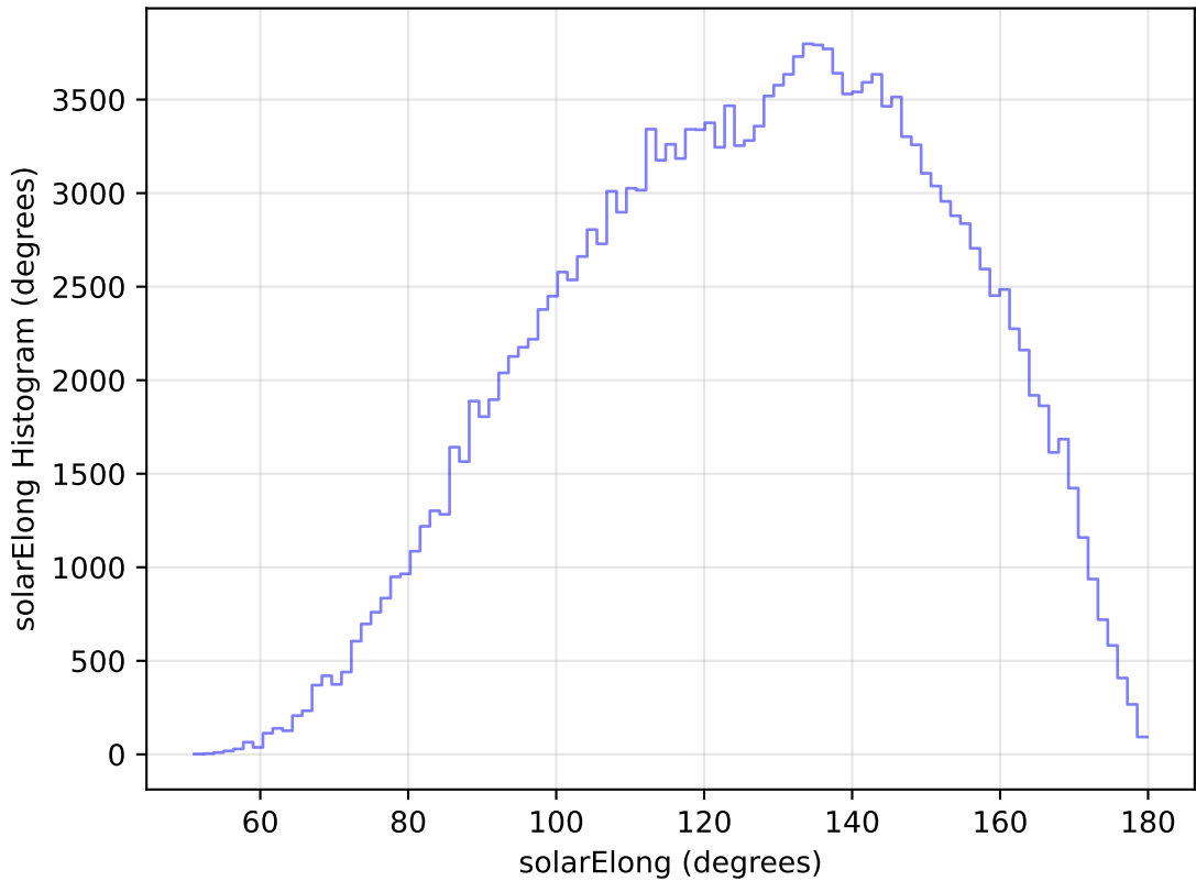
internal_u_expt27_nscale1.0v3.4_10yrs WFD g band: solarElong Histogram
