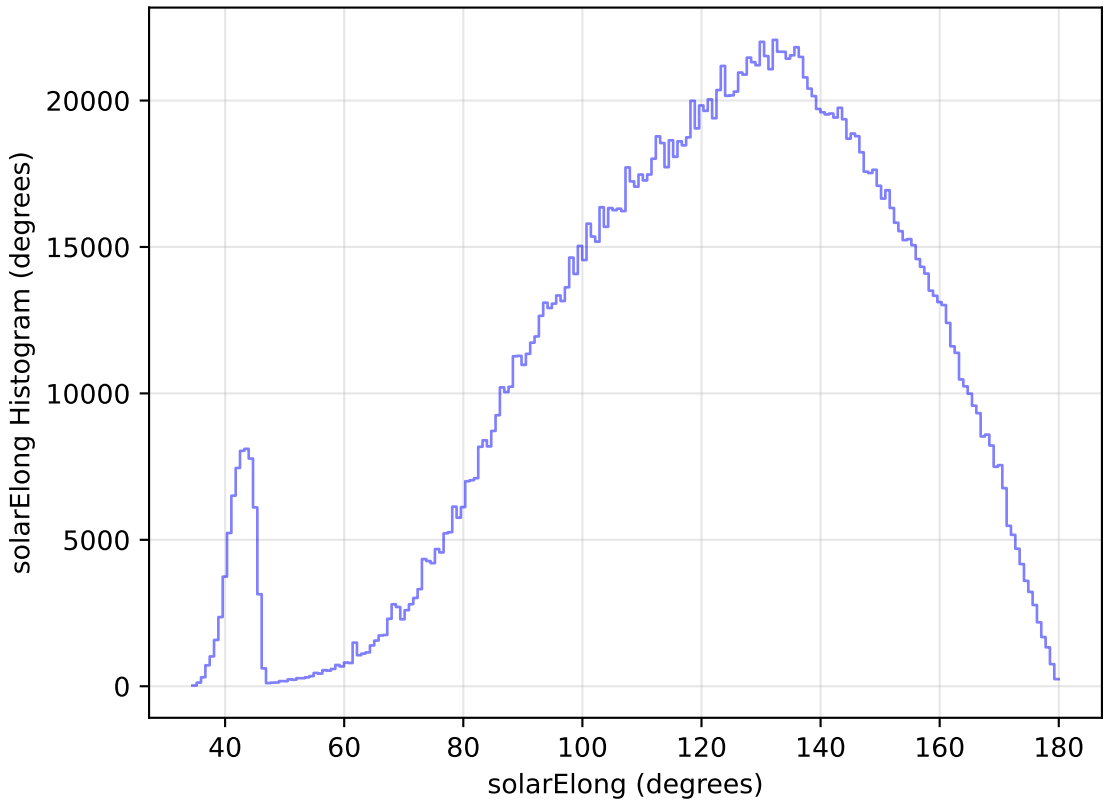
internal_u_expt27_nscale1.0v3.4_10yrs WFD all bands: solarElong Histogram
