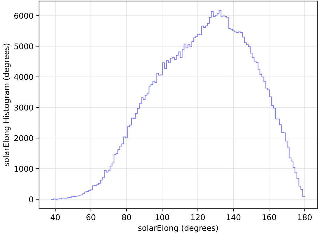
internal_u_expt27_nscale1.0v3.4_10yrs All sky y band: solarElong Histogram
