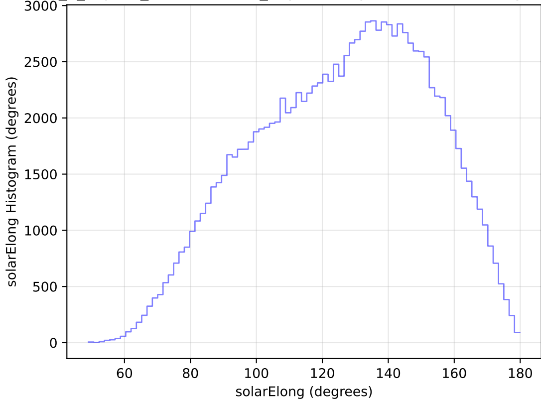
internal_u_expt27_nscale1.0v3.4_10yrs All sky u band: solarElong Histogram
