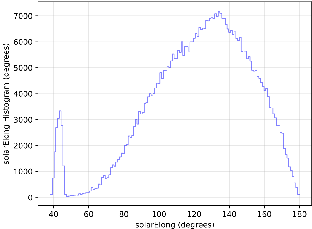
internal_u_expt27_nscale1.0v3.4_10yrs All sky r band: solarElong Histogram
